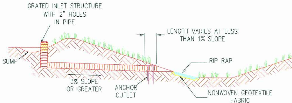
STAND PIPE DROP SPILLWAY MINIMUM COVER OF PIPE = PIPE DIA X 2
