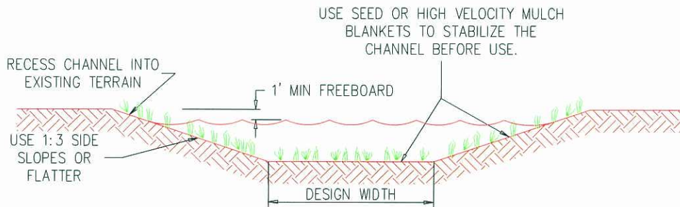
TRAPEZOIDAL CHANNEL VEGETATED SWALE
